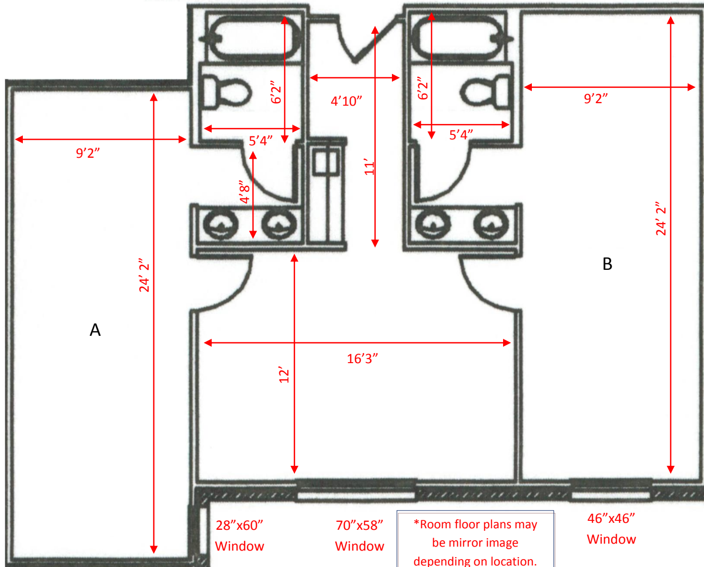
Zink - Allen Floor Plan 7
