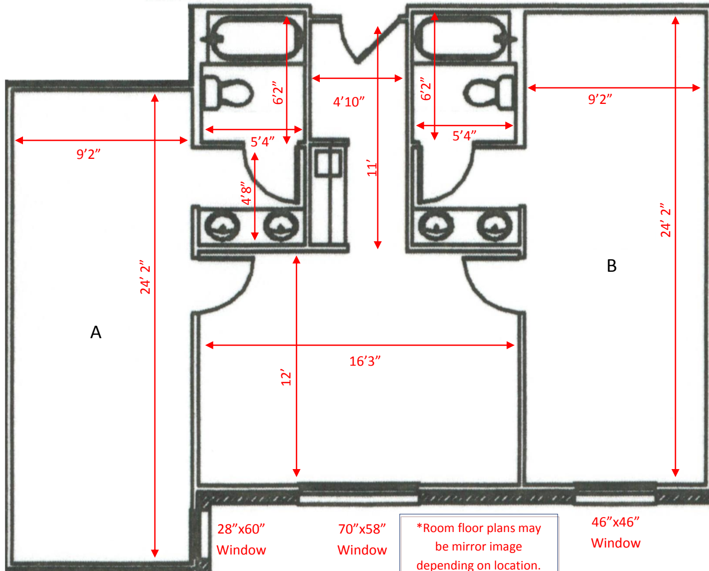
Patchin - Jones Floor Plan 7
